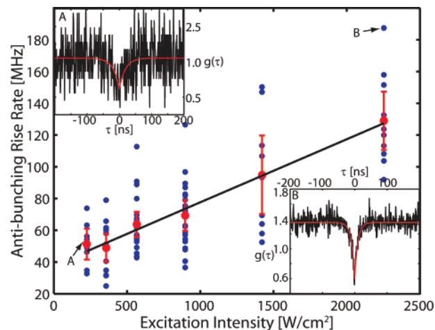
Figure 4. Rise rates \Gamma_e + \tau_f^{-1} (blue circles) as determined from 80 tracked qdots at varied excitation intensities. Red circles with error bars indicate the sample mean. Insets show g^2(\tau) for data points A and B with fits to eq 1.
